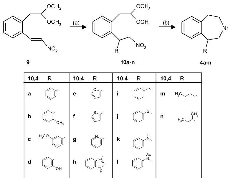
Scheme 2. (a) Various nucleophiles, for details see text. (b) Zn, HCl, THF, reflux.
